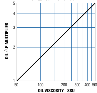
OIL ΔP CORRECTION CURVE
